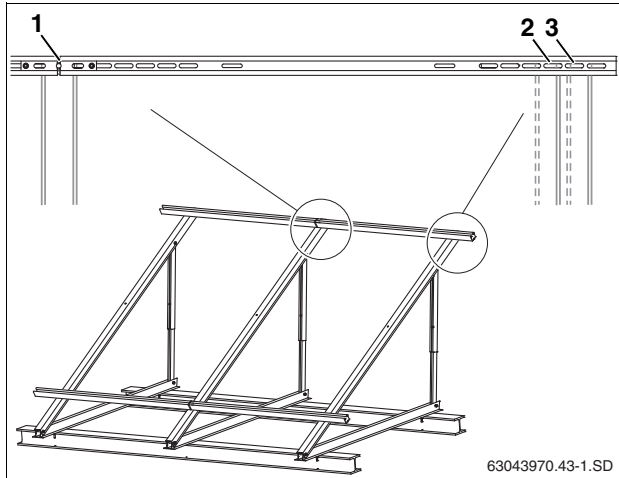
Fig. 32 Aligning the profile rails when connected to the substructure
