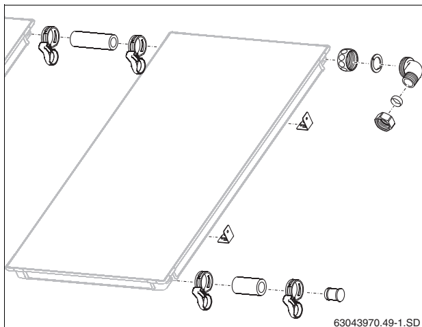
Fig. 64 Fitting the collector sensor and connection parts
