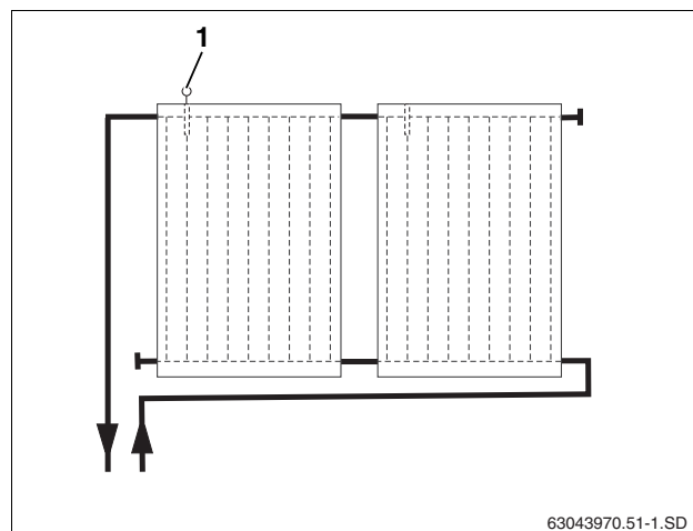
Fig. 41 Water connection – supply line (left)
