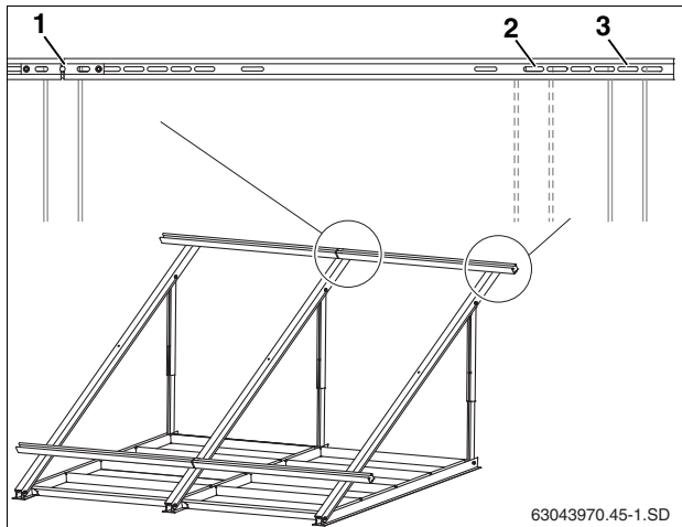
Fig. 33 Aligning the profile rails for ballast trays
