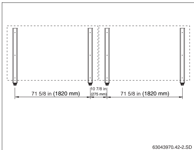
Fig. 21 Basic version for 2 Landscape collectors
