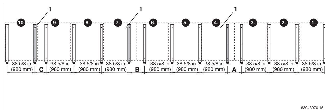
Fig. 23 Basic version for up to 10 Portrait collectors
