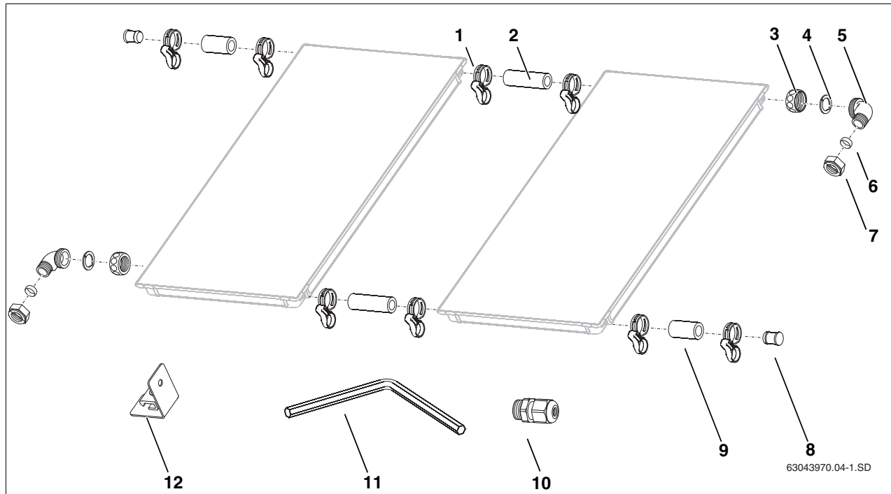
Fig. 4 Connection kit
