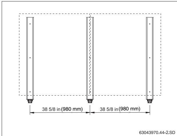
Fig. 19 Basic version for 2 Portrait collectors
