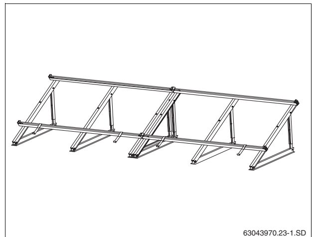
Fig. 18 Flat roof rack for 2 Landscape collectors
