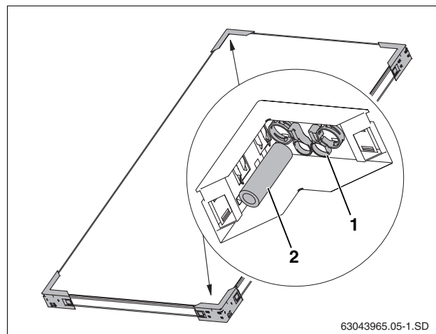
Fig. 5 Two protective corners carry the collector connection sets
