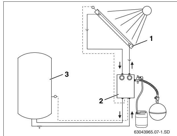
Fig. 7 Solar system components and technical documentation
