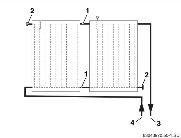
Fig. 40 Water connection – supply pipe (right)
