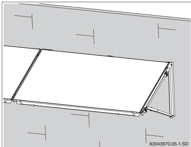
Fig. 38 Wall installation
