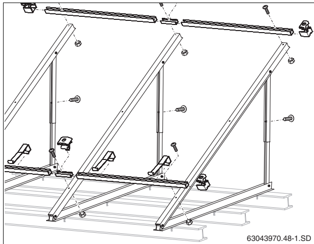
Fig. 62 Installing on a flat roof
