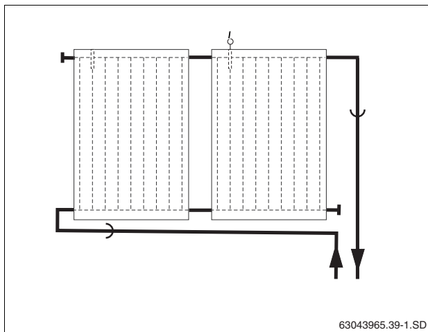
Fig. 63 Water connections
