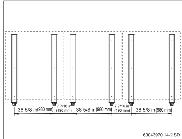
Fig. 22 Auxiliary supports for 3 Portrait collectors
