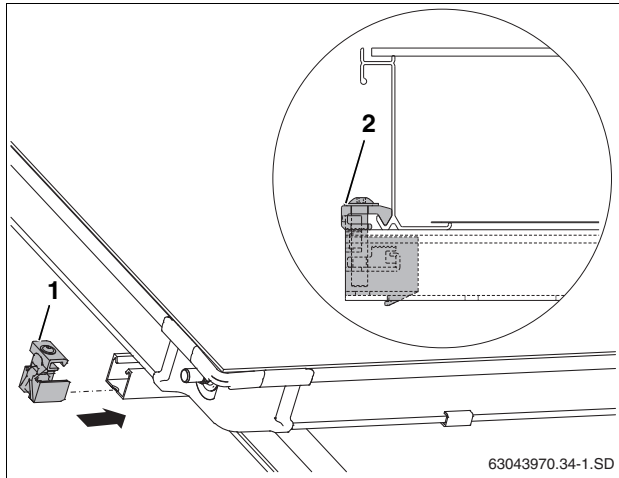
Fig. 52 Single-sided collector clamp (left)
