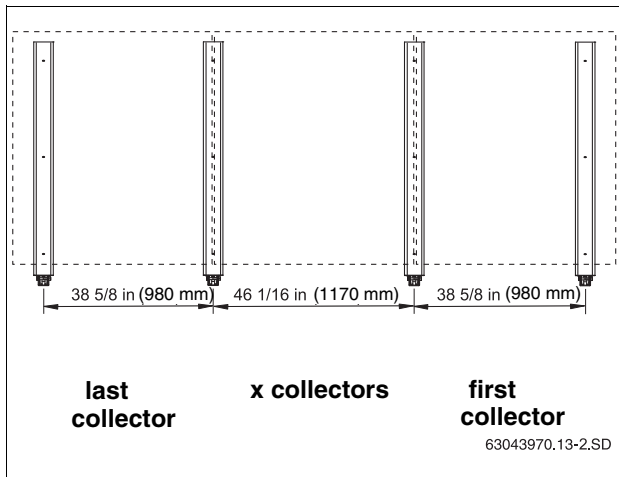
Fig. 20 Basic version for 3 – 10 Portrait collectors
