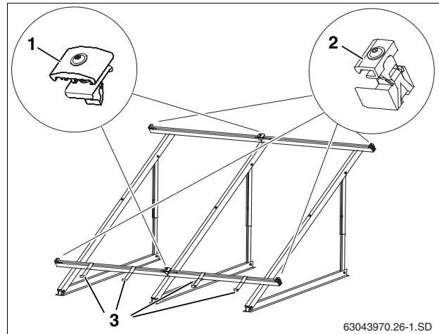
Fig. 44 Fasteners for the collector
