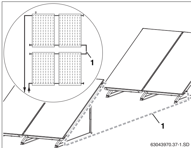
Fig. 61 Two collector arrays, one behind the other
