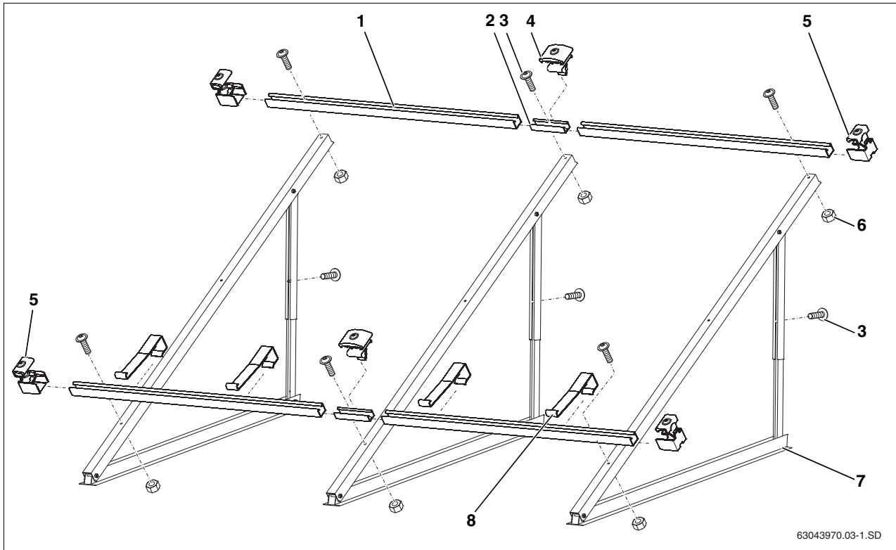
Fig. 3 Rack set for 2 collectors - 1 basic rack, 1 extension rack
