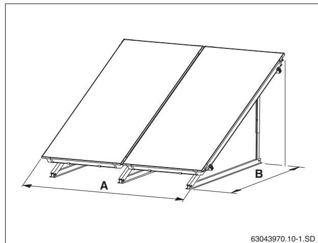
Fig. 16 Space requirements – collector array – Portrait collectors
