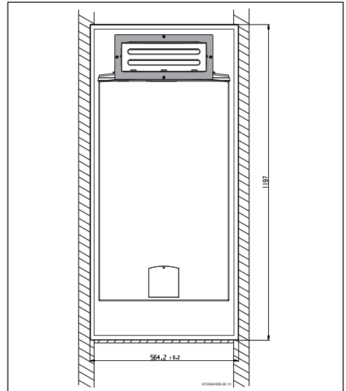
Fig. 11 Mounting the heater inside recess box
