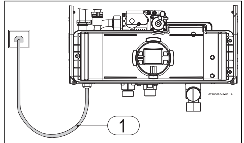
Fig. 22 Connecting power supply cord
