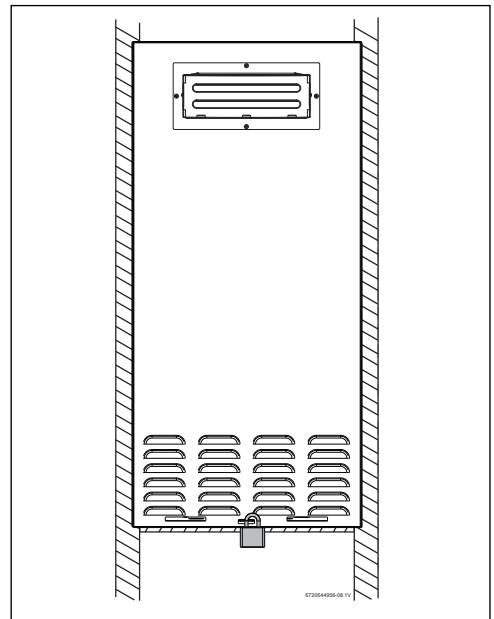
Fig. 12 Close the recess box cover with Padlock
